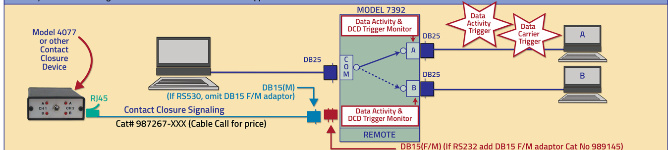
PathWay® Model 7392 Single Channel RS232/RS530 A/B Switch Application w/ Fallback & Remote Control Port
