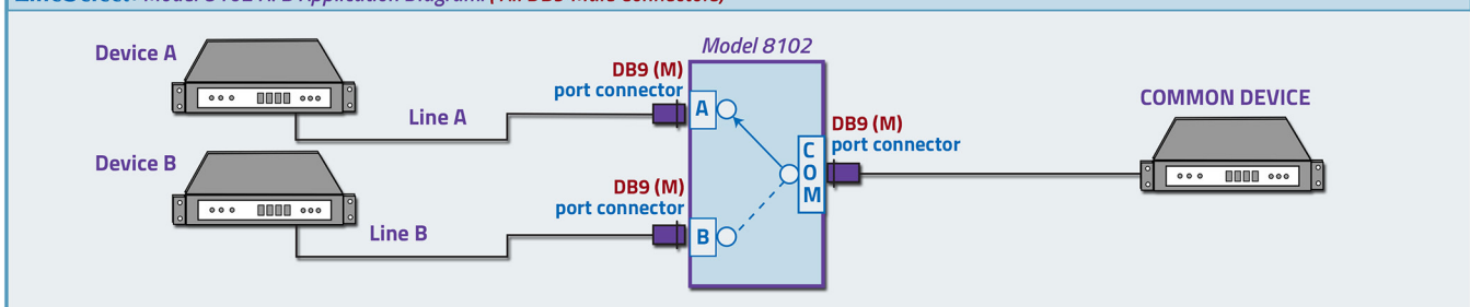
LineSelect® Model 8102 A/B Application Diagram: ( All DB9 Male Connectors)
