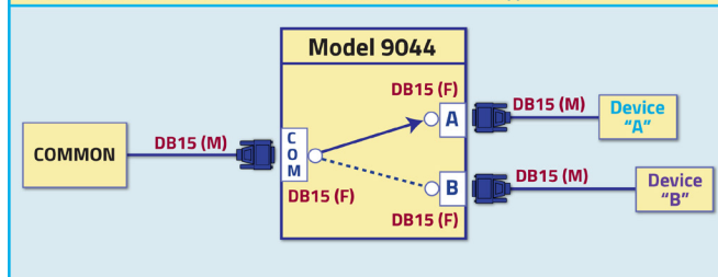
LineSelect® Model 9044 DB15 Manual A/B (FFF) Switch Module Application
