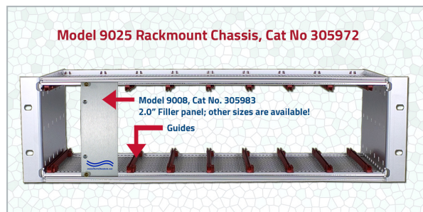
Model 9025 (Cat. No. 305972) Rack Chassis supports Model 9065 (Cat, No. 305444) switch module. Shown here are with optional filler panel. More filler panel sizes available!
