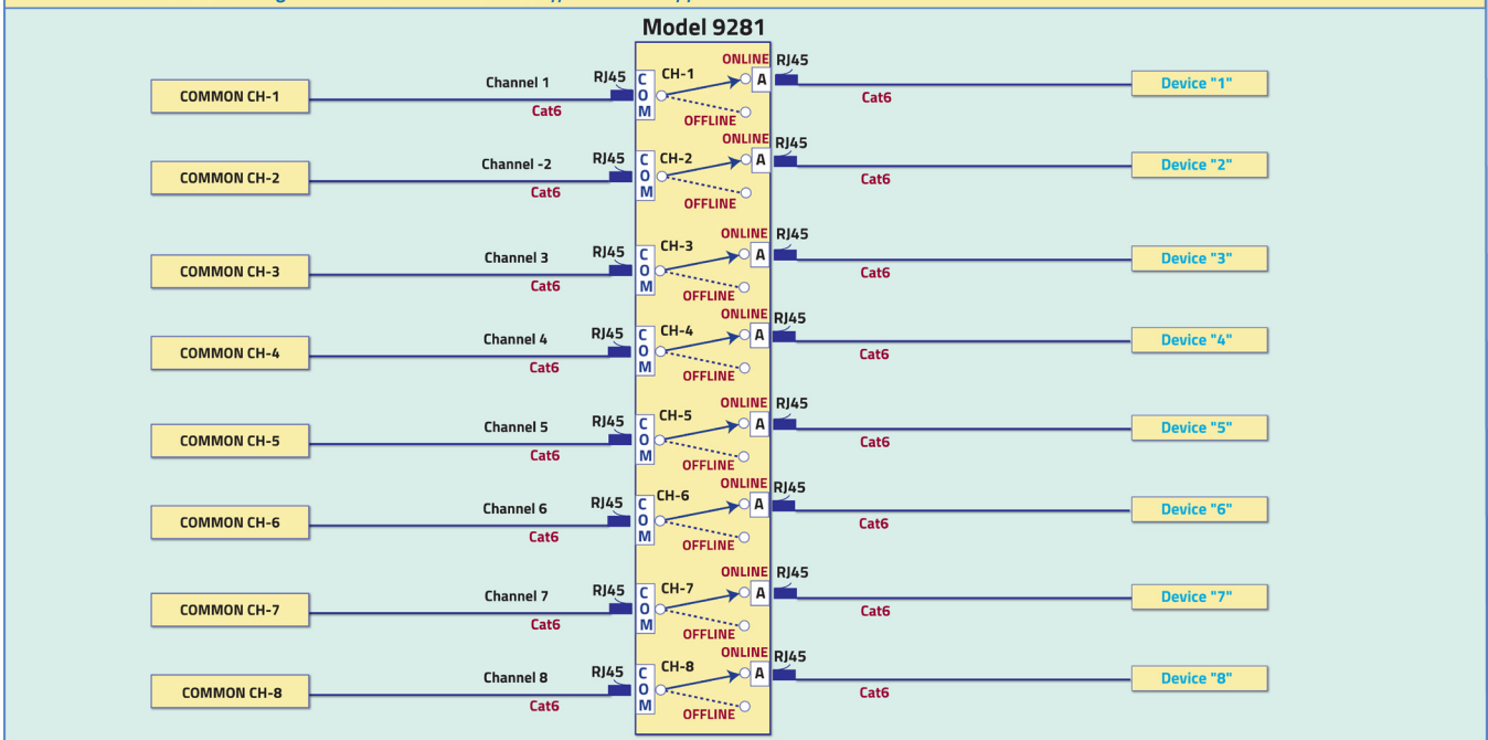
LineSelect® Model 9281 Eight Channel RJ45 Cat6 OnLine/OffLine Switch Application
